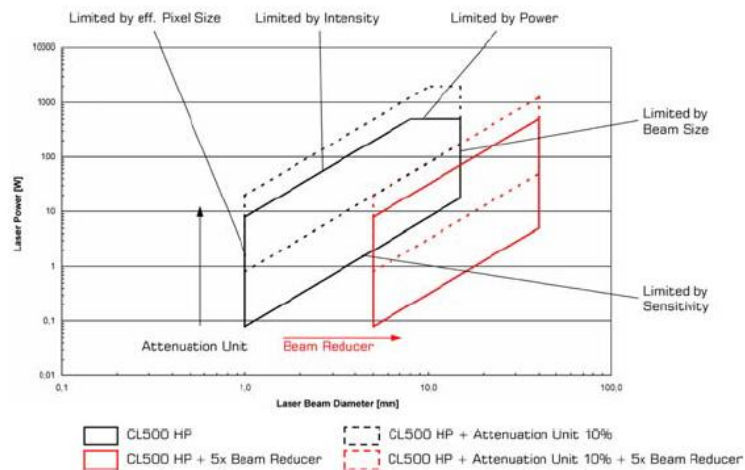
Operational range of LaserDec CL500 HP
